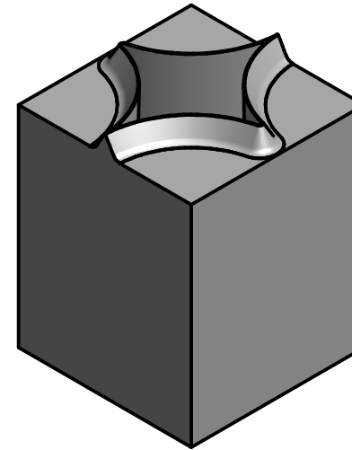
FS1003-1 FULL STAR R9,55 18x18mm, 23,80mm HIGH
