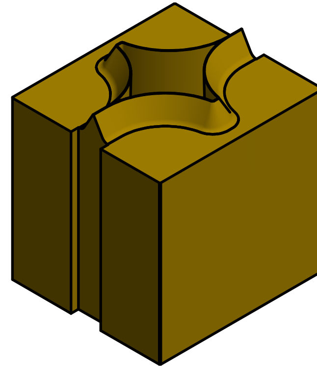
TFS4004-1 FULL STAR R8,00 22x20mm, 23,70mm HIGH TO SUIT 4mm CUTTING RULE TiN COATED
