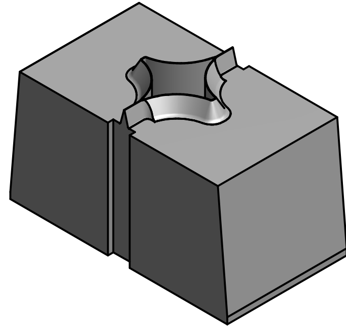
FS4022-1T FULL STAR R8,00 22x40mm, 23,70mm HIGH WITH 5° TAPERED SIDES TO SUIT 4mm CUTTING RULE
