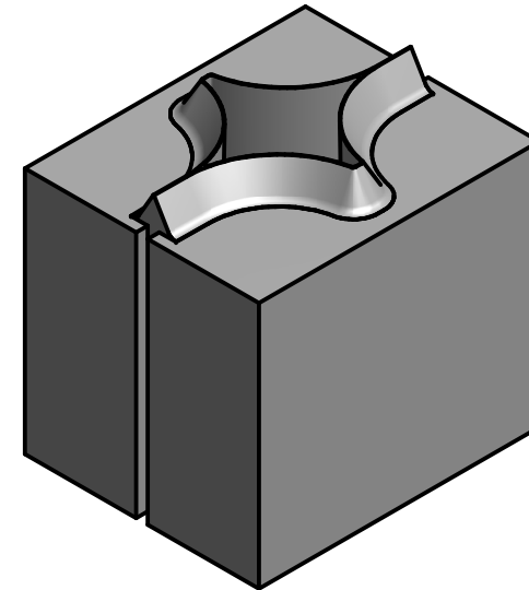
FS1004-1 FULL STAR R8,00 24x20mm, 23,80mm HIGH TO SUIT 1mm CUTTING RULE
