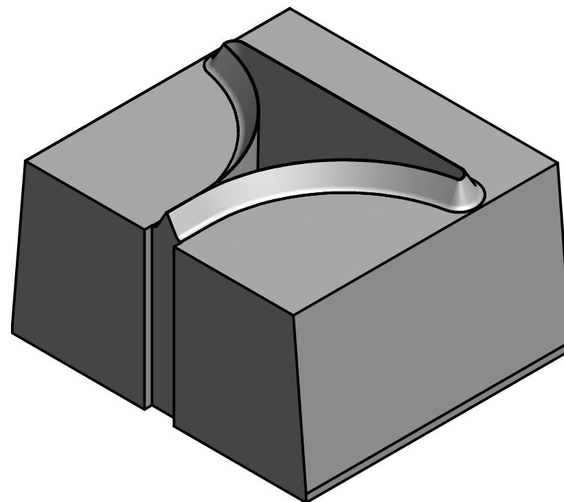
HS3640-2T HALF STAR R20,00 36x40mm, 23,70mm HIGH WITH 5° TAPERED SIDES TO SUIT 4mm CUTTING RULE
