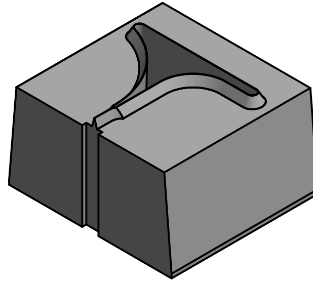
HS4036-4P HALF STAR R20,00 36x40mm, 23,70mm HIGH WITH 5° TAPERED SIDES AND R8,00 PEEL TAB TO SUIT 4mm CUTTING RULE
