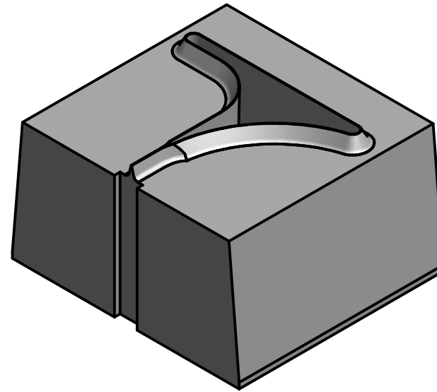
HS4036-20P HALF STAR R20,00 36x40mm, 23,70mm HIGH WITH 5° TAPERED SIDES AND R8,00 PEEL TAB TO SUIT 4mm CUTTING RULE
