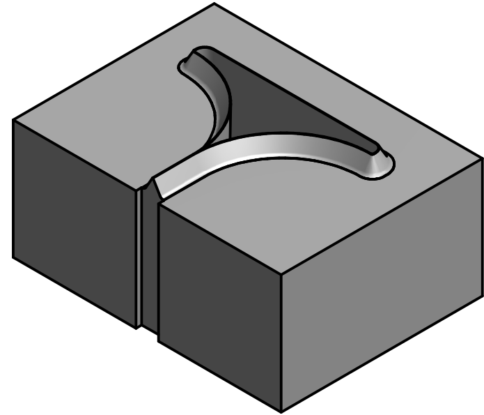
HS4836-2 HALF STAR R16,00 36x48mm, 23,80mm HIGH TO SUIT 4mm CUTTING RULE
