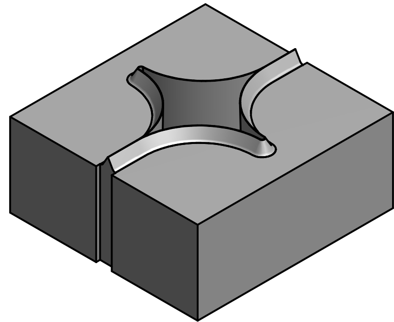
FS5048-1 FULL STAR R16,00 50x48mm, 23,80mm HIGH TO SUIT 4mm CUTTING RULE
