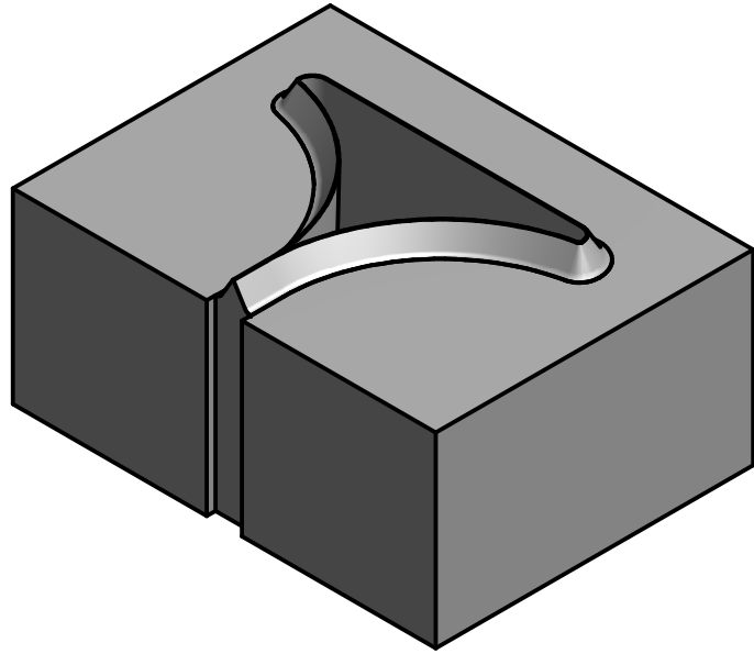
HS4836-4 HALF STAR R20,00 36x48mm, 23,70mm HIGH TO SUIT 4mm CUTTING RULE
