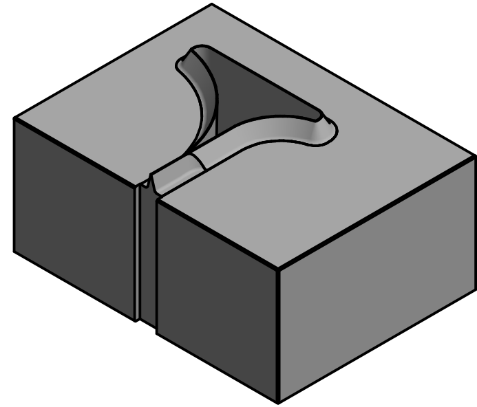
HS4836-4P HALF STAR R20,00 36x48mm, 23,70mm HIGH WITH R9,00 PEEL TAB TO SUIT 4mm CUTTING RULE
