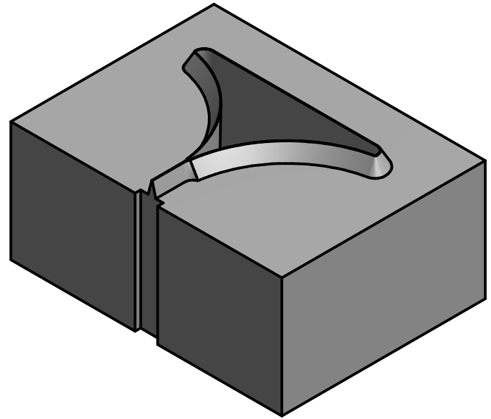
HS4836-20 HALF STAR R20,00 36x48mm, 23,70mm HIGH TO SUIT 4mm CUTTING RULE
