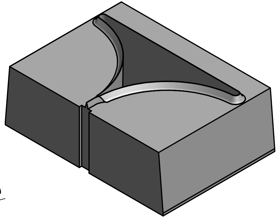
HS6546-30 HALF STAR R30,00 46x65mm, 23,70mm HIGH WITH 5° TAPERED SIDES TO SUIT 4mm CUTTING RULE
