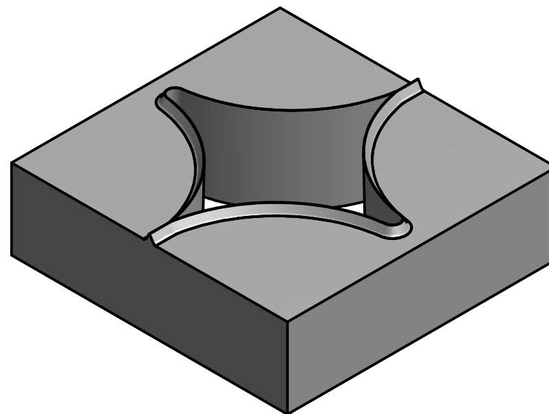
FS7573-1 FULL STAR R35,00 73x75mm, 23,80mm HIGH
