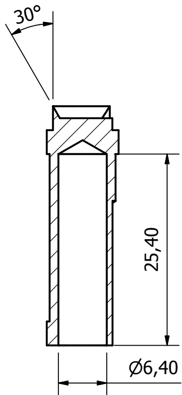
SECTION BY-BY
