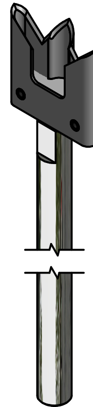
EP0530-1 EUROPUNCH ON A SHAFT \varnothing 4,90 \times 29,90 mm, 175mm HIGH
