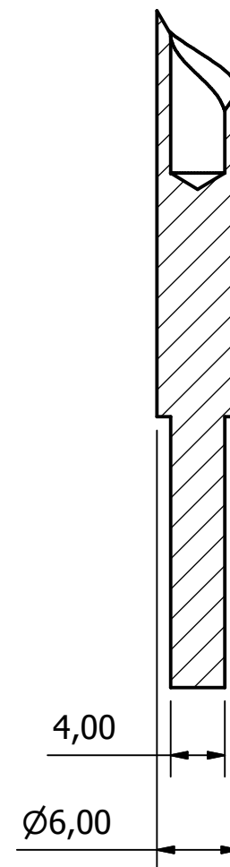
SECTION X-X
