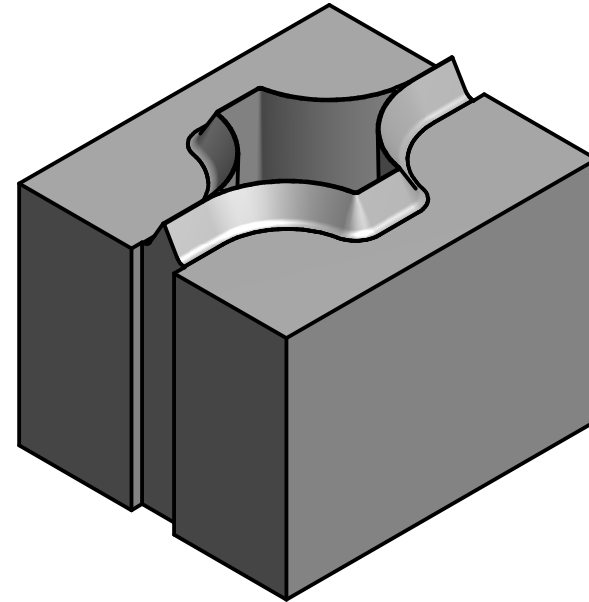
FS2925-1 FULL STAR R8,00 29x25mm, 23,70mm HIGH TO SUIT 4mm CUTTING RULE
