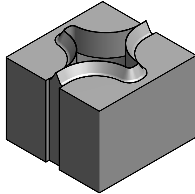
FS2928-R10 FULL STAR R10,00 29x28mm, 23,70mm HIGH TO SUIT 4mm CUTTING RULE
