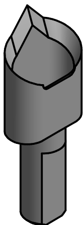
AP3312-30 OVAL AIR PUNCH 12x6mm x 33mm LONG WITH FLATS
