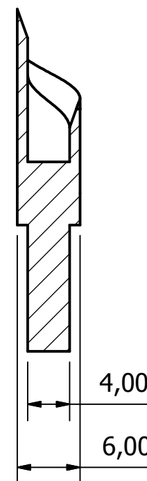
SECTION X-X
